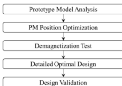
Figure 2. Computation steps
