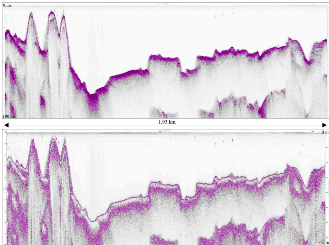
Figure 5. Cross-section of HRSP MC03 before (top) and after processing (bottom) - Viewing position according to Figure 1
