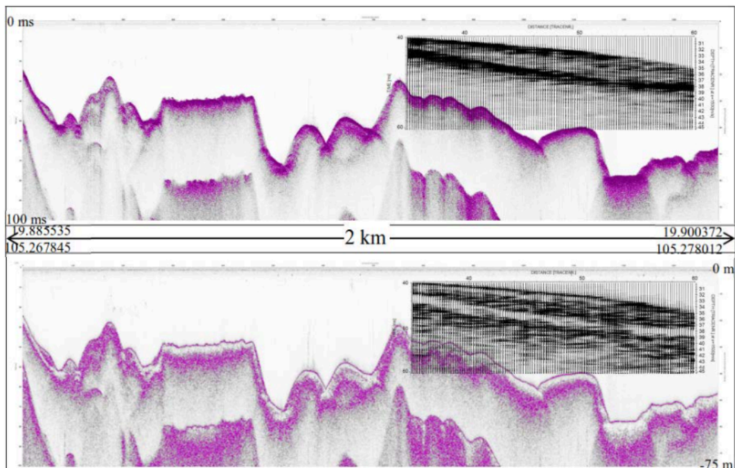
Figure 4. Cross-section of HRSP MC02 before (top) and after processing (bottom) - Viewing position according to Figure 1
