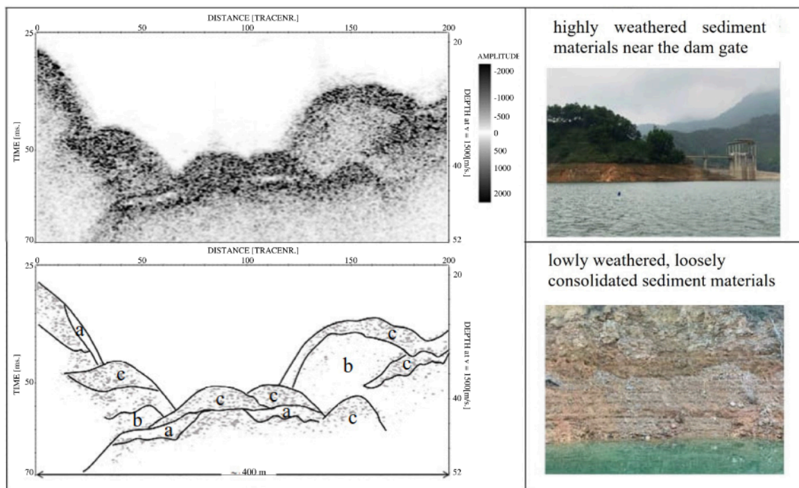
Figure 10. Sectional excerpt from MC01 and the main acoustic reflection boundaries
