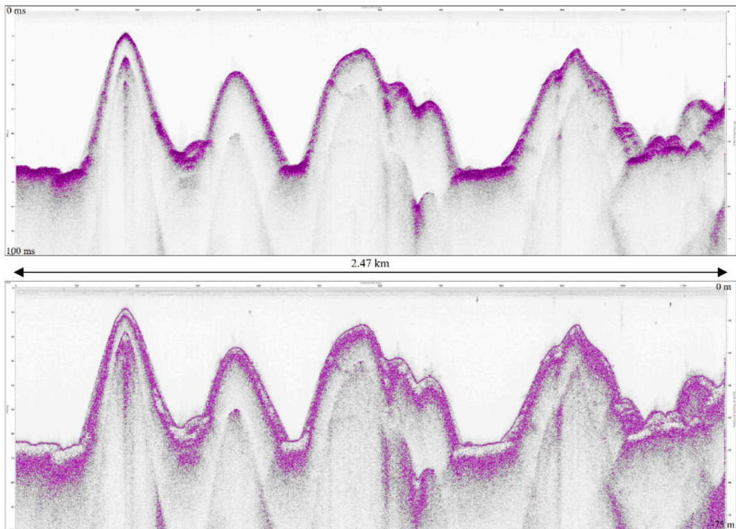
Figure 3. Cross-section of HRSP MC01 before (top) and after processing (bottom) - Viewing position according to Figure 1
