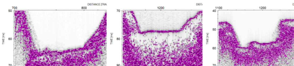
Figure 9. U-shaped terrain type with a flat bottom due to redeposition on cross-sections MC01, MC02, and MC03 (from left to right)
