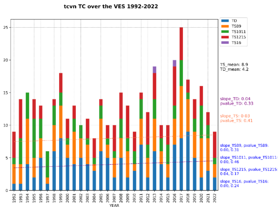
Figure 3. Annual Numbers of Tropical Depression (TD), Tropical Storm Force 8–9 (TS89), Severe Tropical Storm Force 10–11 (TS1011), Typhoons Force 12–15 (TS1215), và Super Typhoons Force 16 or higher (TS16) based on the Beaufort Scale active over the EVS during 1992–2022. TS mean and TD mean respectively represent the calculated average of tropical storms and tropical depressions. “slope” and “pvalue” suggest the statistical trend and significant level based on the Theil Sen-Kendall methodology
