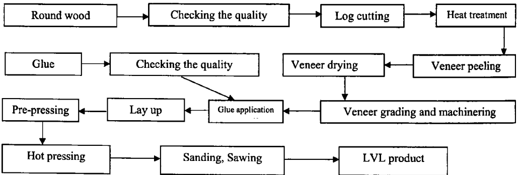
Figure 01. Technical process of producing LVL
