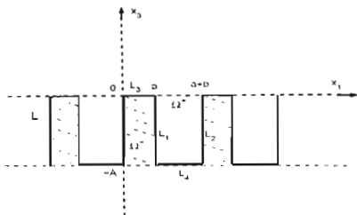
Fig. 1. Two-dimensional domains \Omega^+ and \Omega^- are separated by a very rough interface L of comb-type ( 0 < a + b \ll A ).
